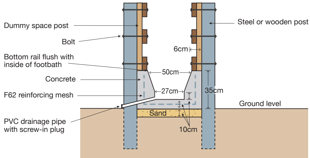
Figure 4b: Main features of a walk-through footbath — elevation (top) (not to scale)
