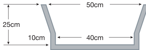
Figure 3: Main features of a portable footbath — cross-section (not to scale)
