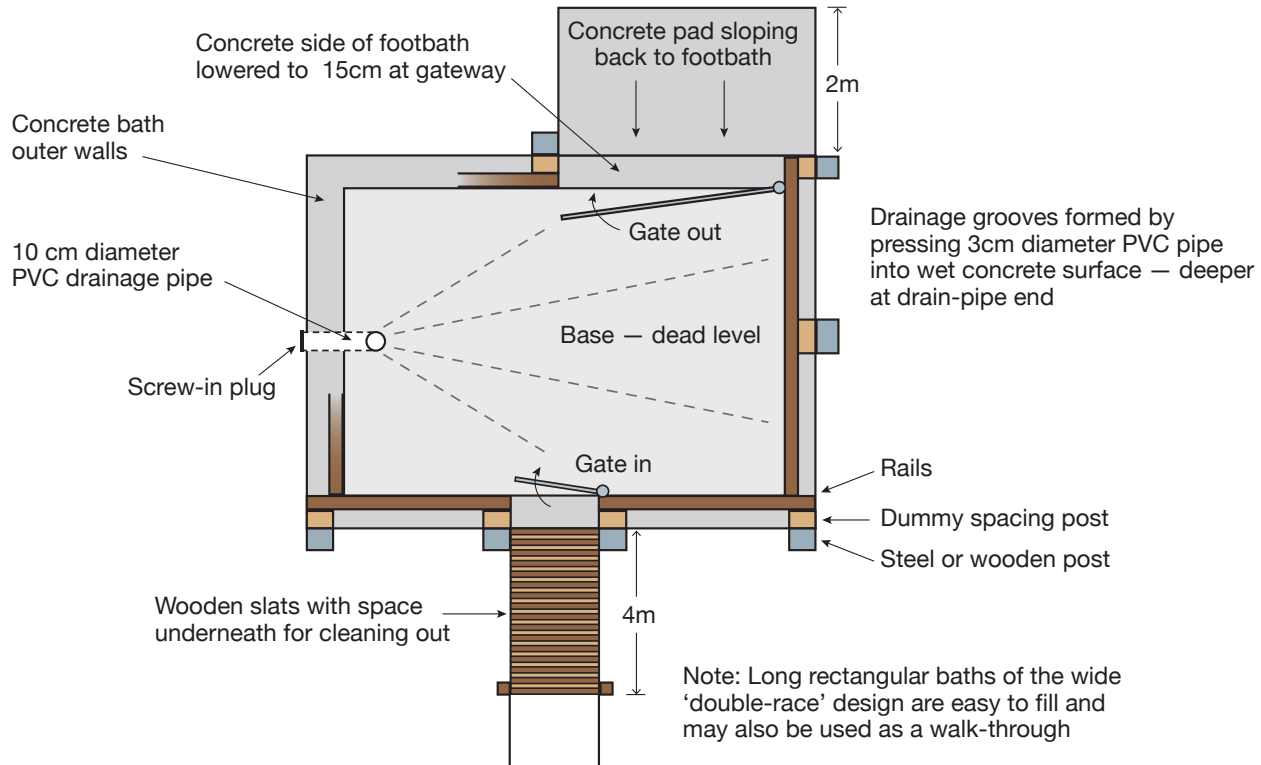
Figure 2(b): Main features of a stand-in footbath — plan (not to scale)
