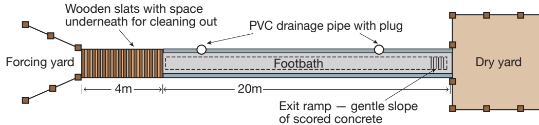
Figure 4a: Main features of a walk-through footbath — plan (not to scale)
