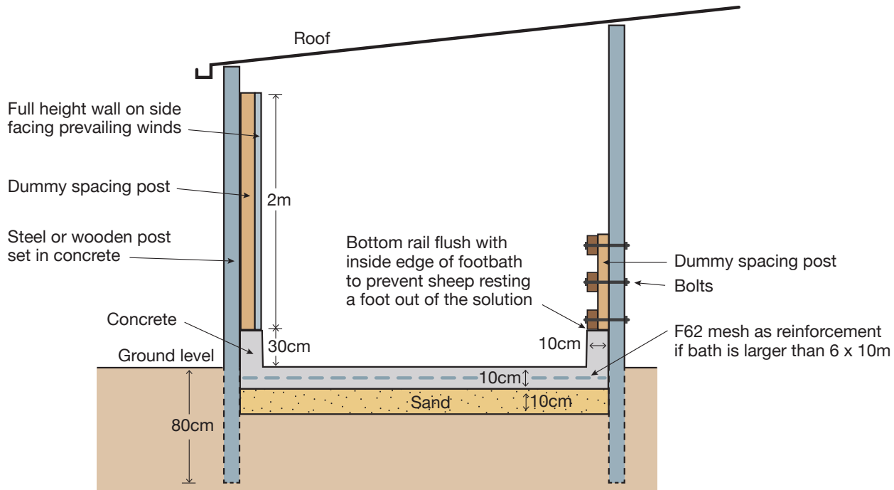
Figure 2a: Main features of a stand-in footbath — elevation (not to scale)
