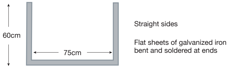
Figure 3: Main features of a portable footbath — cross-section (not to scale)
