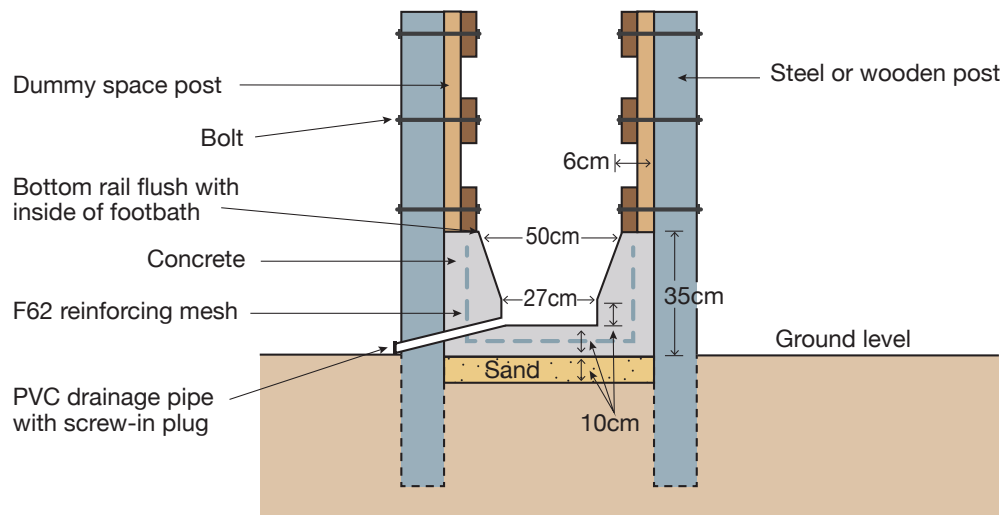
Figure 4b: Main features of a walk-through footbath — elevation (not to scale)
